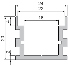
Support profile for LED stripes
